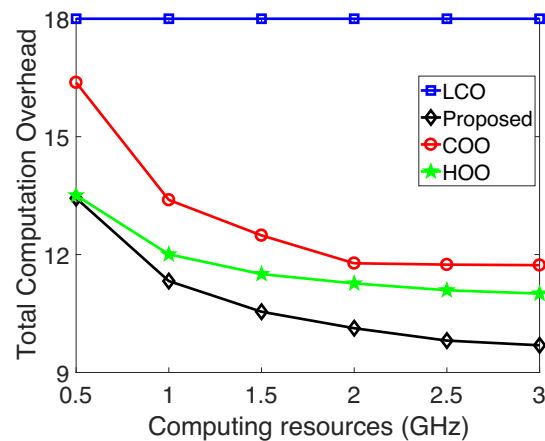
Fig. 8: Comparison of total computation overhead among four schemes under variant remote computing resources.
