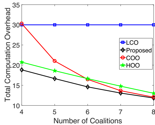
Fig. 7: Comparison of total computation overhead among four schemes under different numbers of coalitions.
