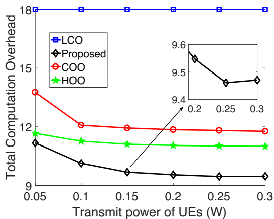
Fig. 9: Comparison of total computation overhead among four schemes under different transmit power of UEs.
