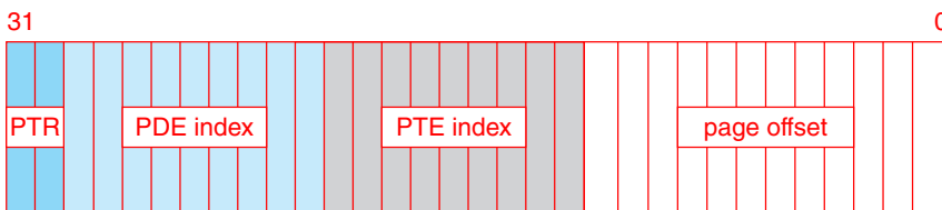
Figure B.4 Virtual-to-physical address translation on IA-32.
