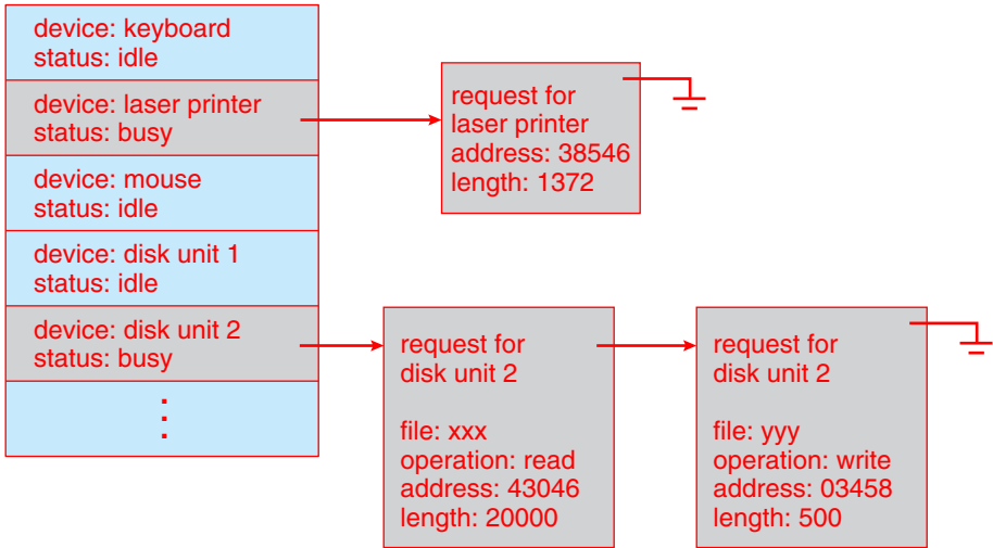
Figure 12.10 Device-status table.
