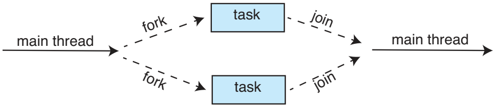
Figure 4.16 Fork-join parallelism.
