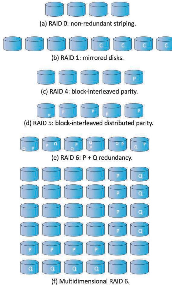
Figure 11.15 RAID levels.
