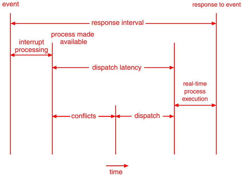
Figure 5.19 Dispatch latency.
