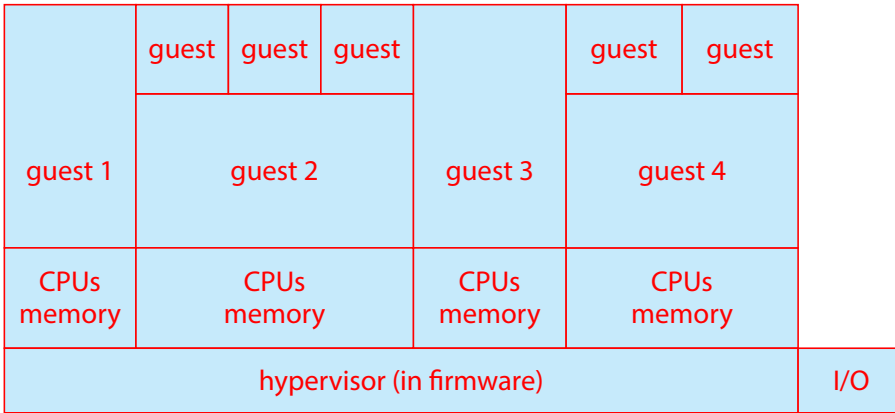
Figure 18.5 Type 0 hypervisor.
