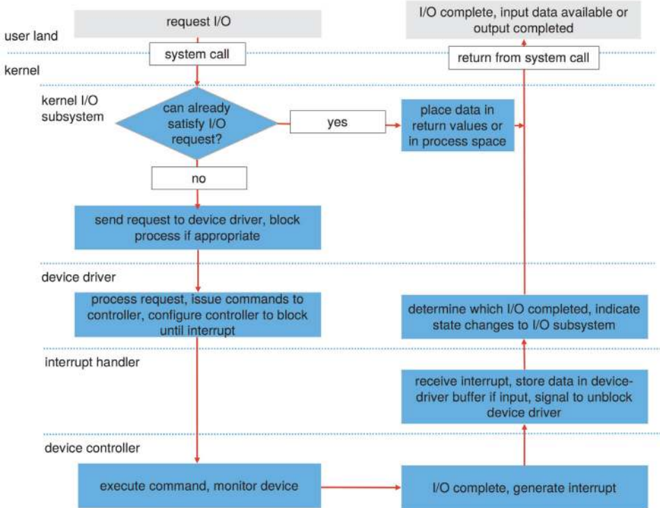
Figure 12.14 The life cycle of an I/O request.
