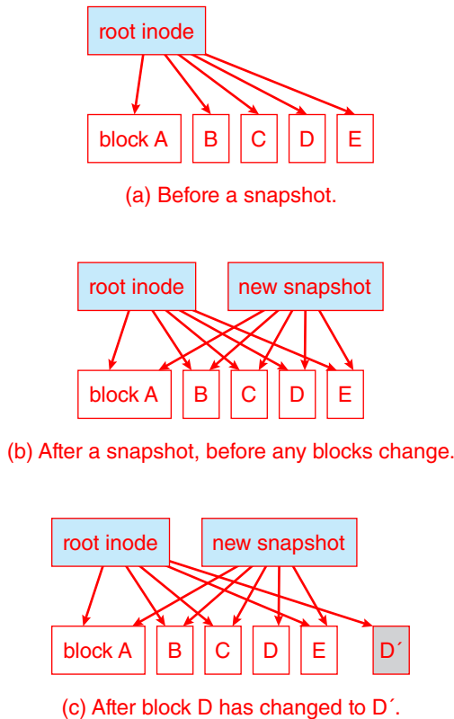
Figure 14.13 Snapshots in WAFL.
