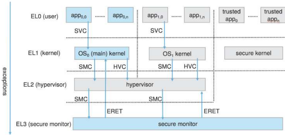
Figure 17.3 ARM architecture.
