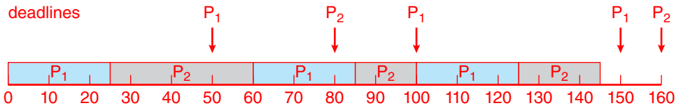
Figure 5.24 Earliest-deadline-first scheduling.
