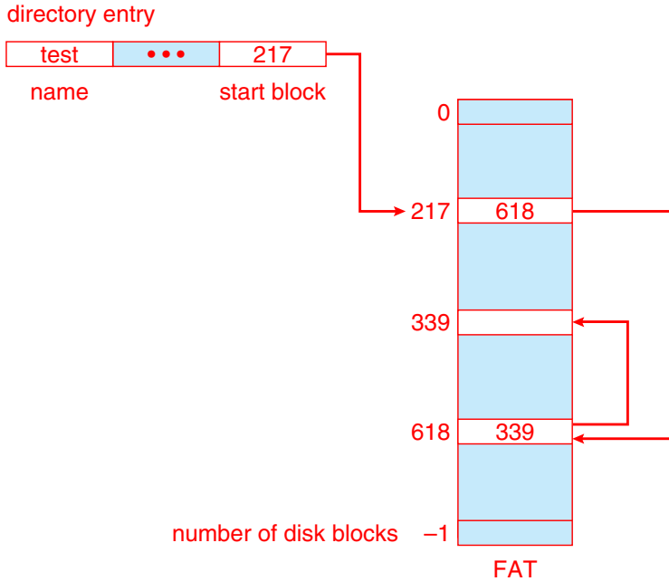
Figure 14.6 File-allocation table.
