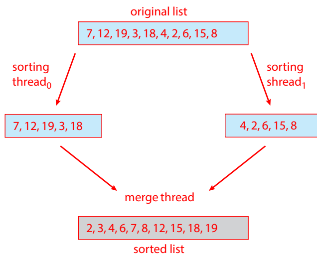
Figure 4.27 Multithreaded sorting.
