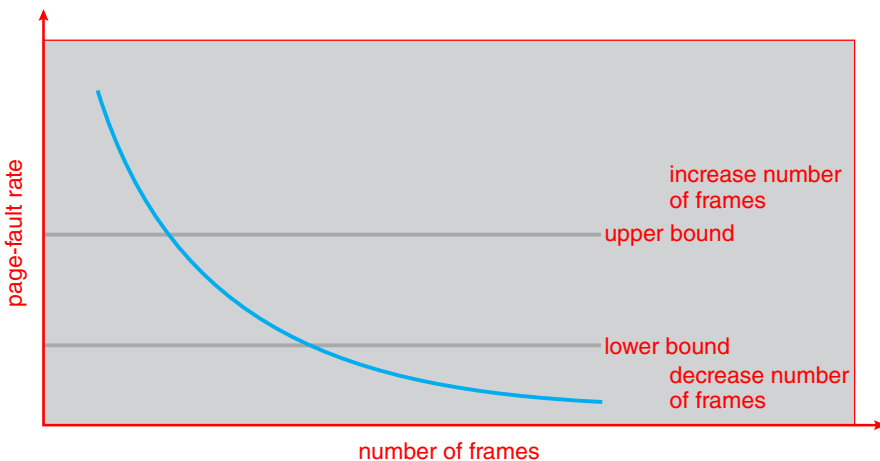
Figure 10.23 Page-fault frequency.
