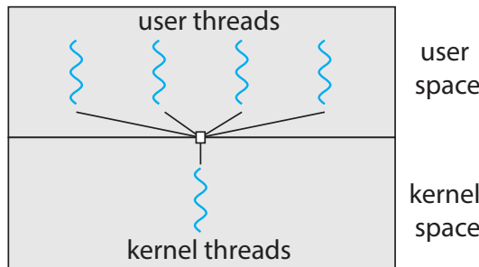
Figure 4.7 Many-to-one model.
