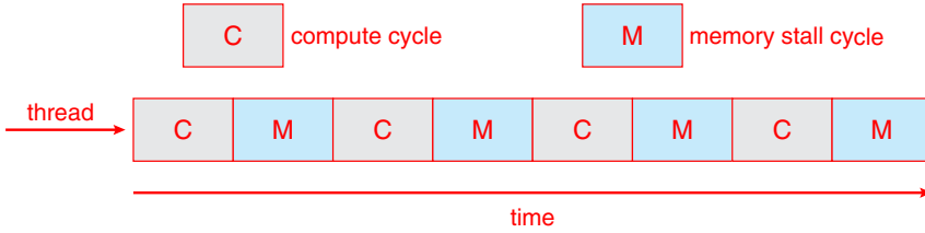
Figure 5.12 Memory stall.
