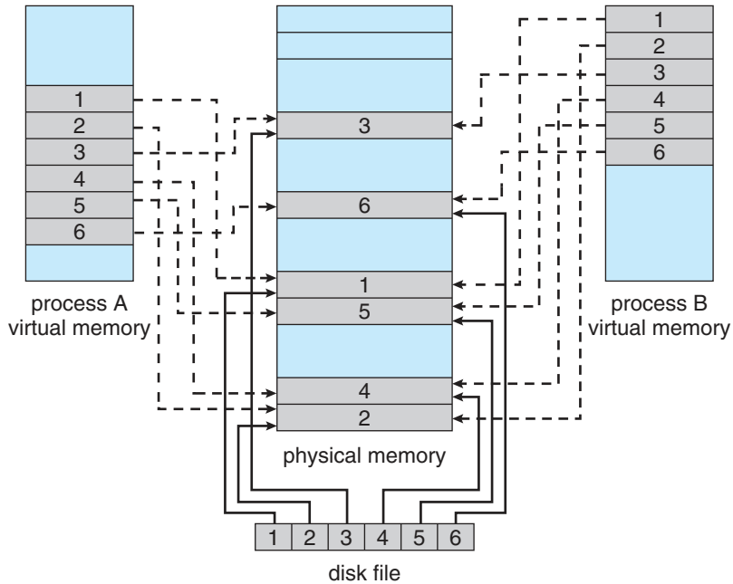
Figure 13.13 Memory-mapped files.
