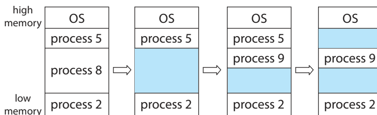
Figure 9.7 Variable partition.
