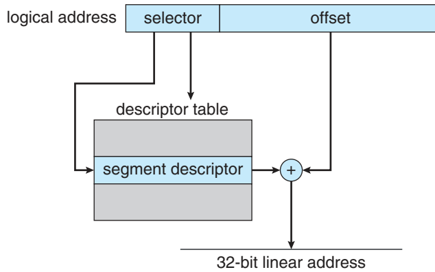
Figure 9.22 IA-32 segmentation.
