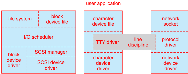
Figure 20.8 Device-driver block structure.
