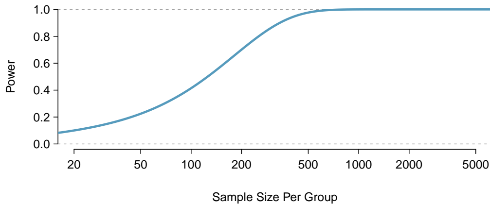
Figure 7.18: The curve shows the power for different sample sizes in the context of the blood pressure example when the true difference is -3 . Having more than about 250 to 350 observations doesn't provide much additional value in detecting an effect when \alpha = 0.05 .
